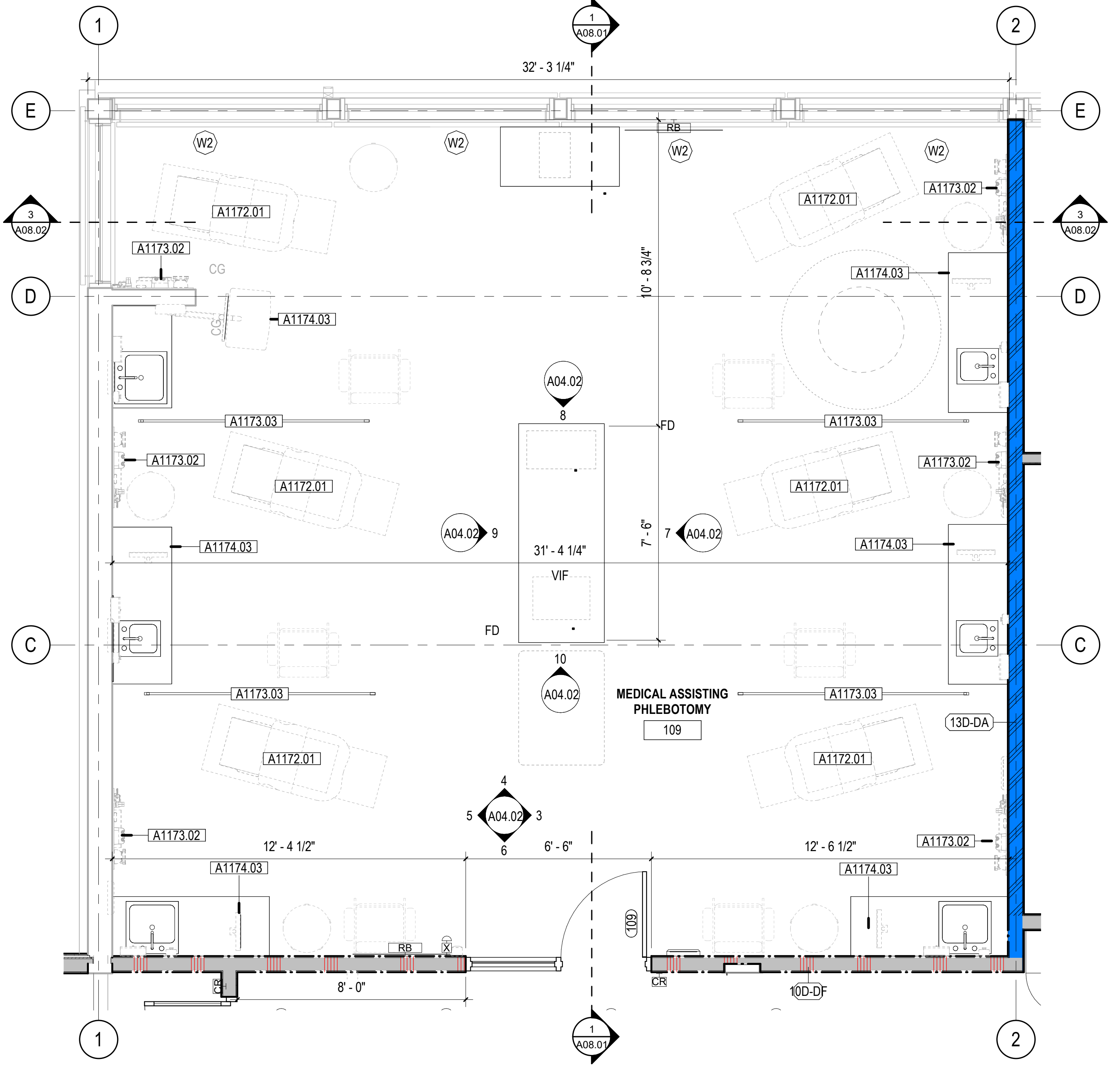
1 ENLARGED PLAN - MEDICAL ASSISTING PHLEBOTOMY 109 3/8" = 1'-0"
