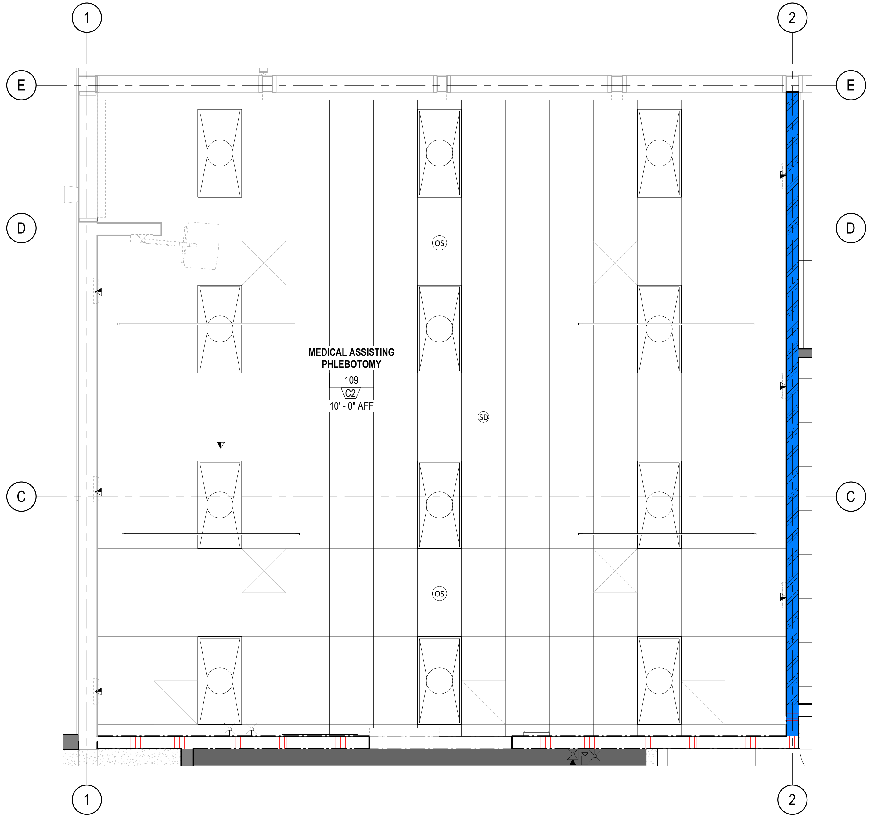
2 ENLARGED REFLECTED CEILING PLAN - MEDICAL ASSISTING PHLEBOTOMY 109 3/8" = 1'-0"
